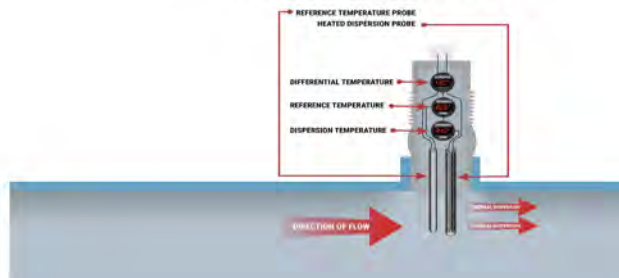
THERMAL DISPERSION FLOW SWITCH
