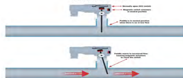
PADDLE TYPE FLOW SWITCH
